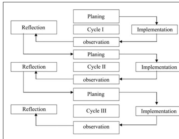
Figure 1: Research cycle.
